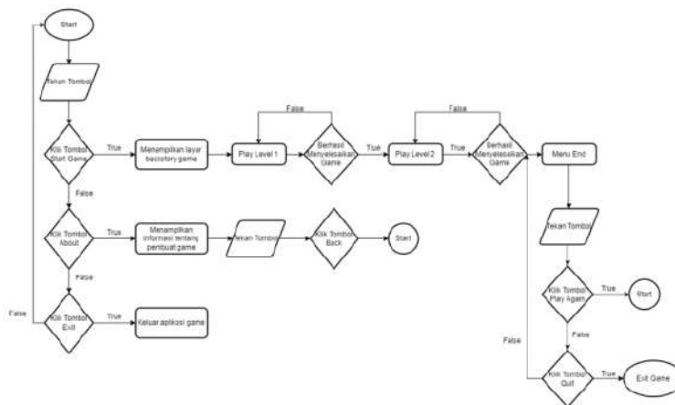
Gambar 4. Flowchart Sistem
