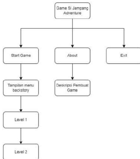
Gambar 3. Rancangan Menu Game
