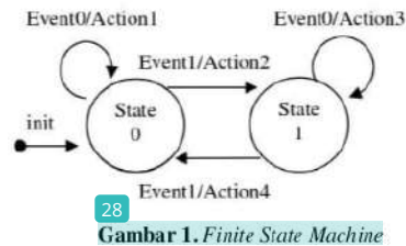
Gambar 1. Finite State Machine
