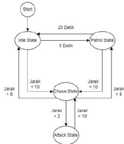
Gambar 2. Implementasi Finite State Machine
